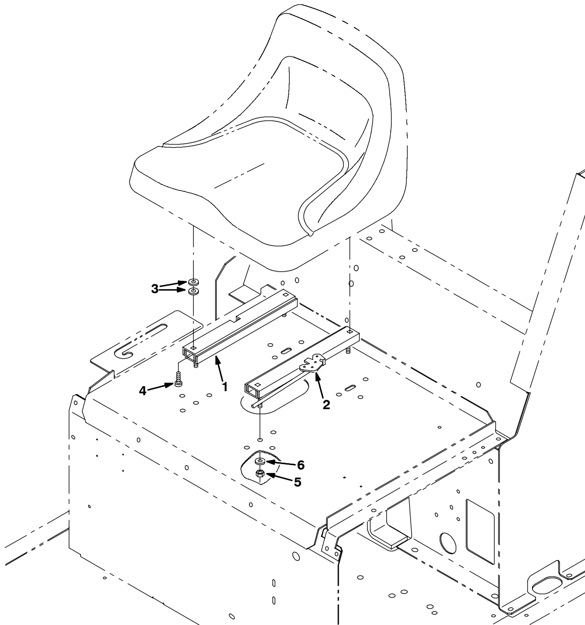
FIG. 1 - SLIDE RAIL KIT INSTALLATION
